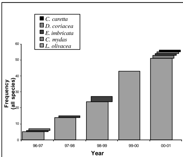
Figure 1: Year wise record of dead sea turtle on St. Martin's island during 1996-2001 due to fishing activity
