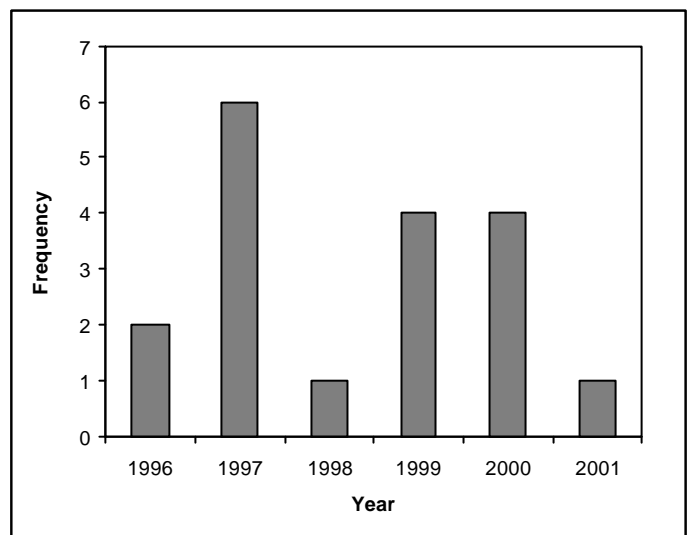
Figure 2: Predation on sea turtle nests on St. Martin's Island by stray dogs during October 1996-June 2001
